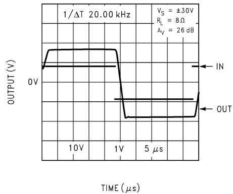
Pulse Response
